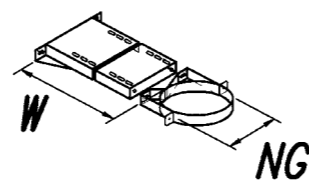
6 Wandhalter W = 200 - 500 mm
