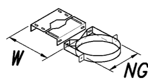
5 Wandhalter W = 70 - 200 mm
