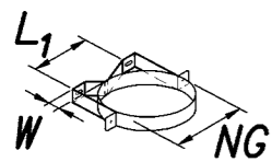
4 Wandhalter W = 50 - 66 mm HAL 9.15.13
