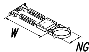
8 Wandhalter W = 268 - 500 mm
