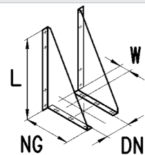
1 Wandkonsole W = 50 - 66 mm, W = 100 - 130 mm HAL 9.20.13 - 23
